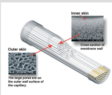
One way filter cartridge Einweg Membranfilter
