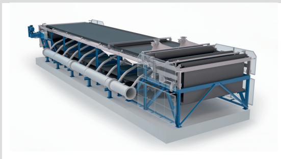
Horizontal vacuum belt filter Horizontale Vakuumbandfilter
